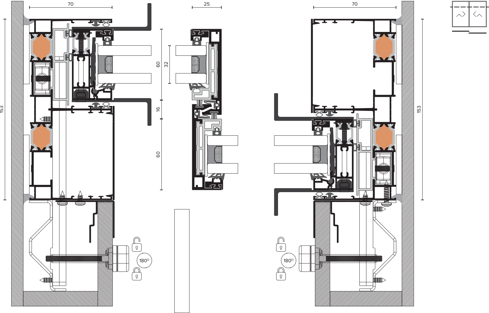
SYMMETRIC LOCK POSITION
