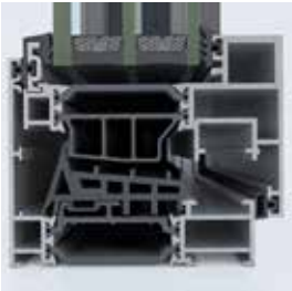
Level 1 *Uf: ≥1.9 W/m²K
