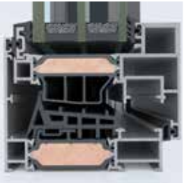
Level 2 *Uf: ≥1.5 W/m²K
