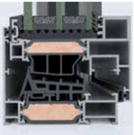
Level 3 *Uf: ≥1.4 W/m²K
